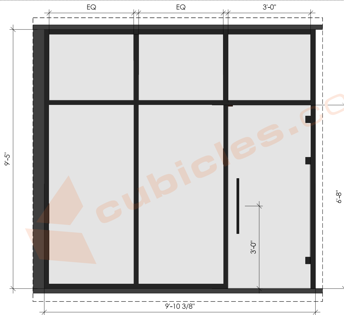
A Office 2 - Elevation 5 Not to Scale
